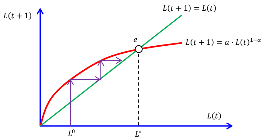
Fig. 1. Population dynamics and population steady state
